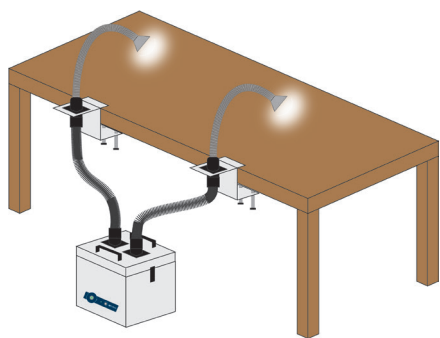
Example setup on FumeCube Dual Arm
